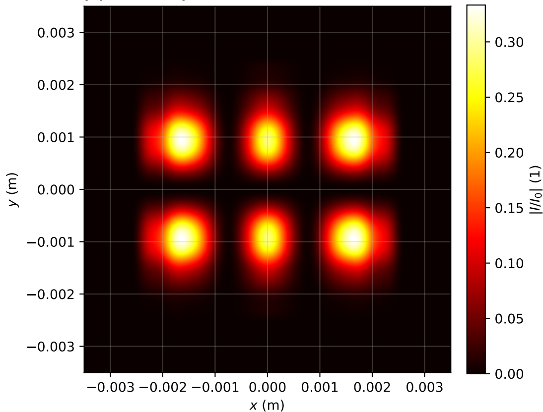
Intensity profile I(x, y, z = 3.582)/I_0 , P_{in}=2.0P_{cr} , artificial time
